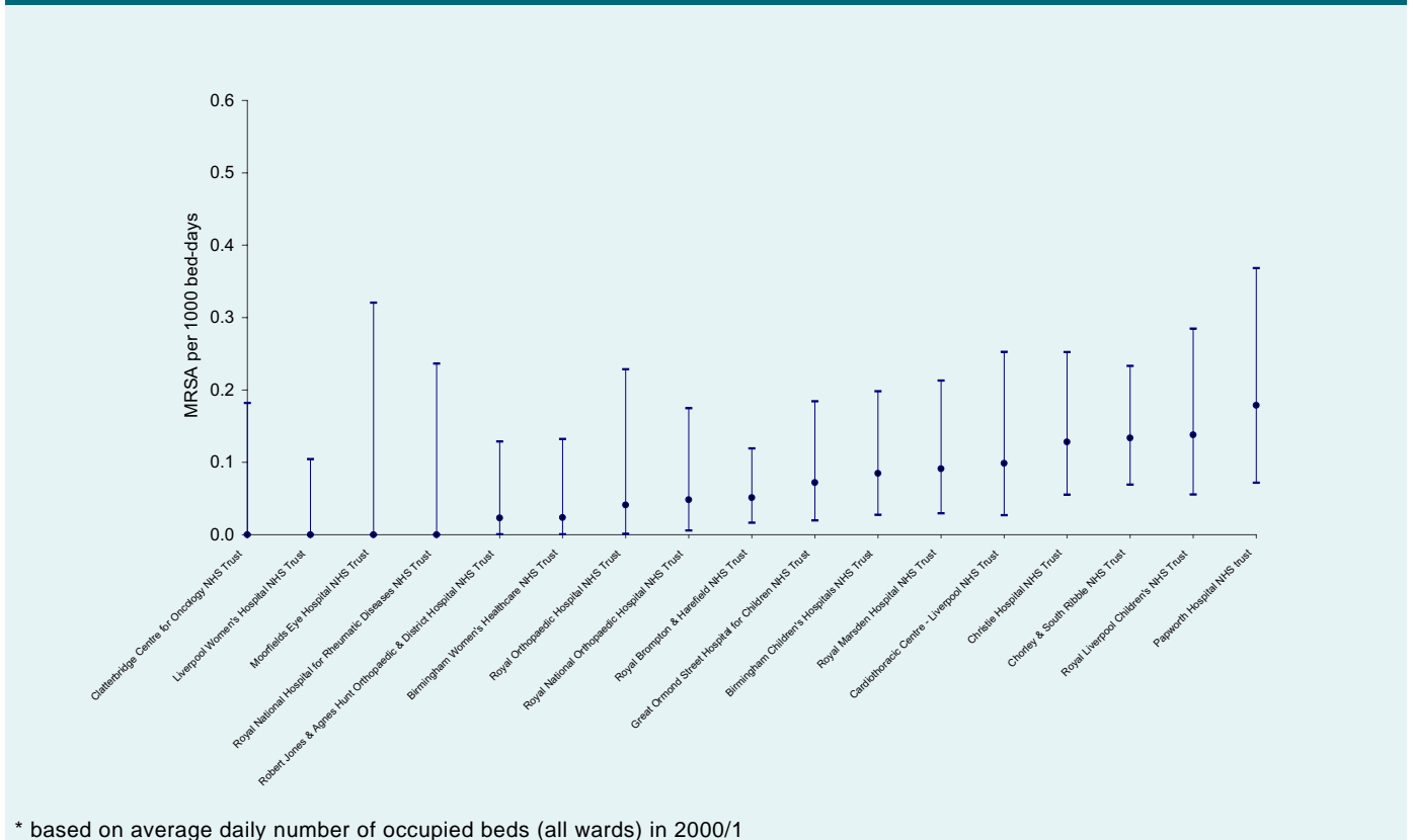
Figure 7 MRSA bacteraemia rates* with 95% confidence intervals, in single speciality trusts: April to December 2001
