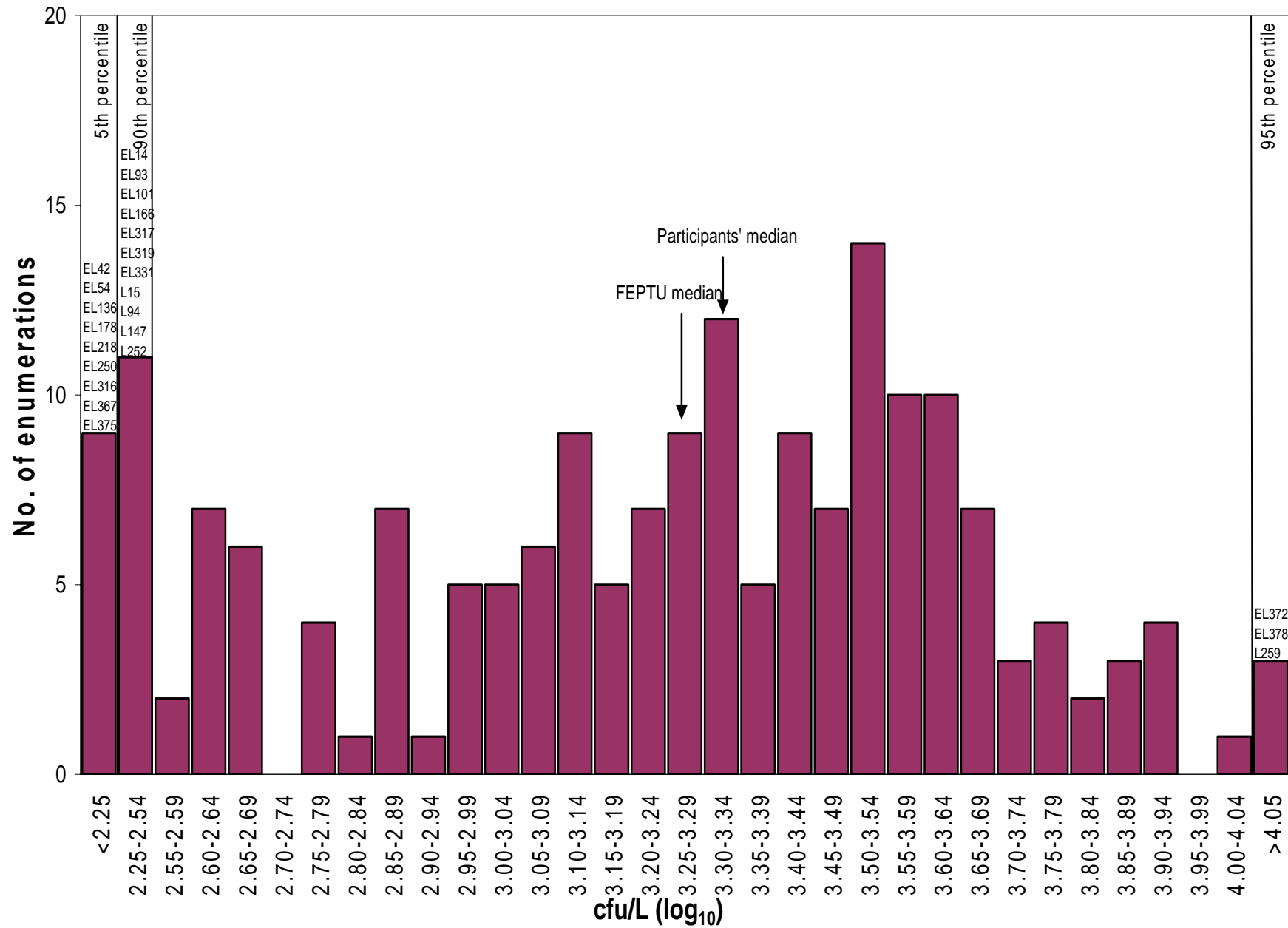
Fig. 2: Log 10 Total Legionella counts reported by participants - sample G63B
