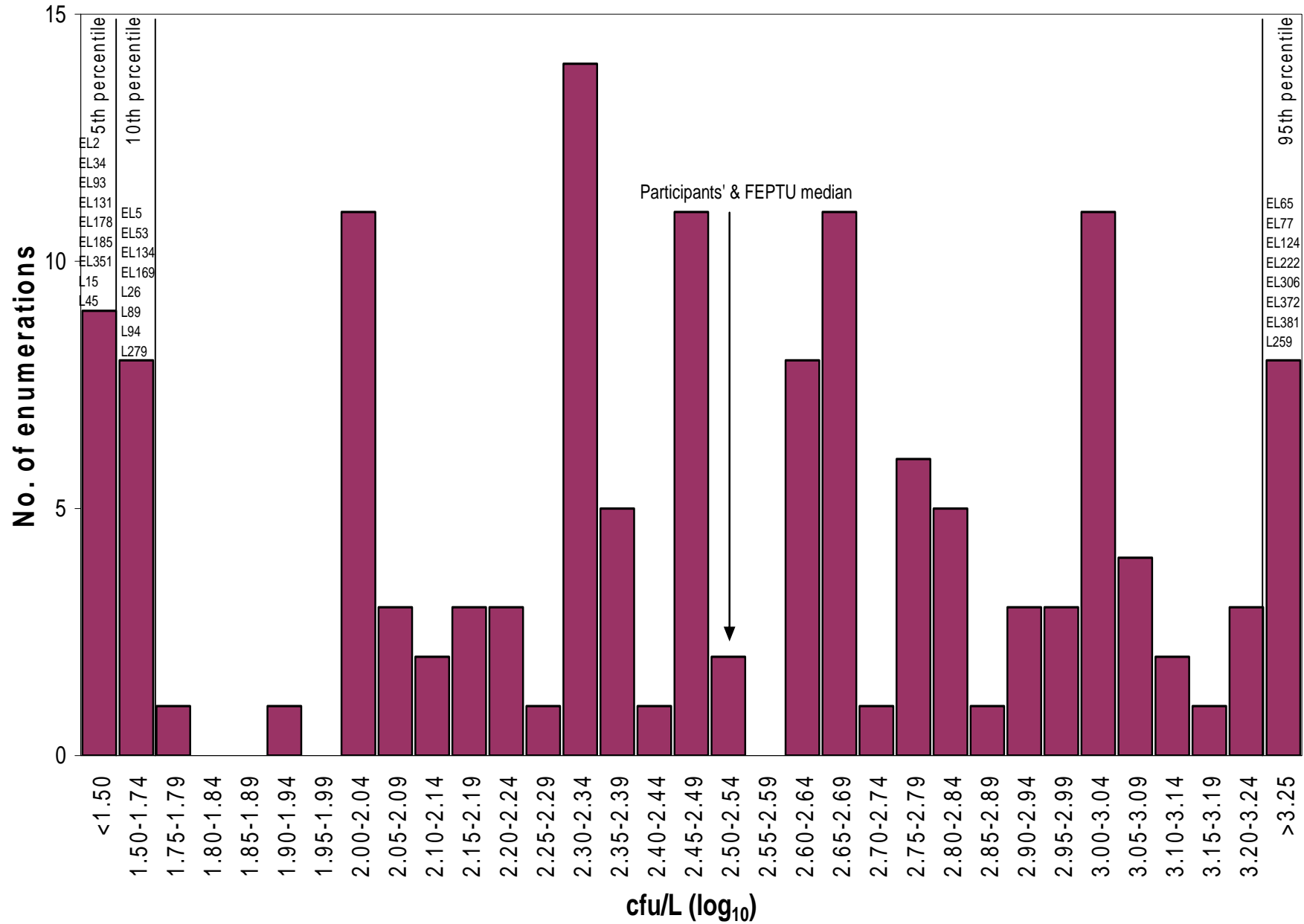
Fig. 1: Log 10 Legionella counts reported by participants - sample G63A
